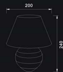
ITEM NO: LS-CHT103 SIZE: \phi 20 \times 24 cm INNER BOX: 23x23x25cm CBM: 0.079m 3 /6pcs
